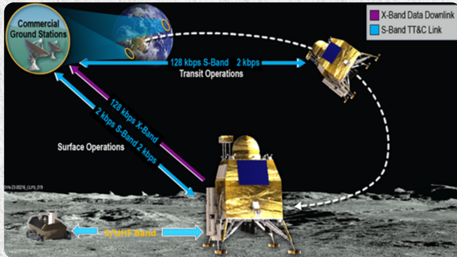
Figure 7:LLV-RF Communication links
