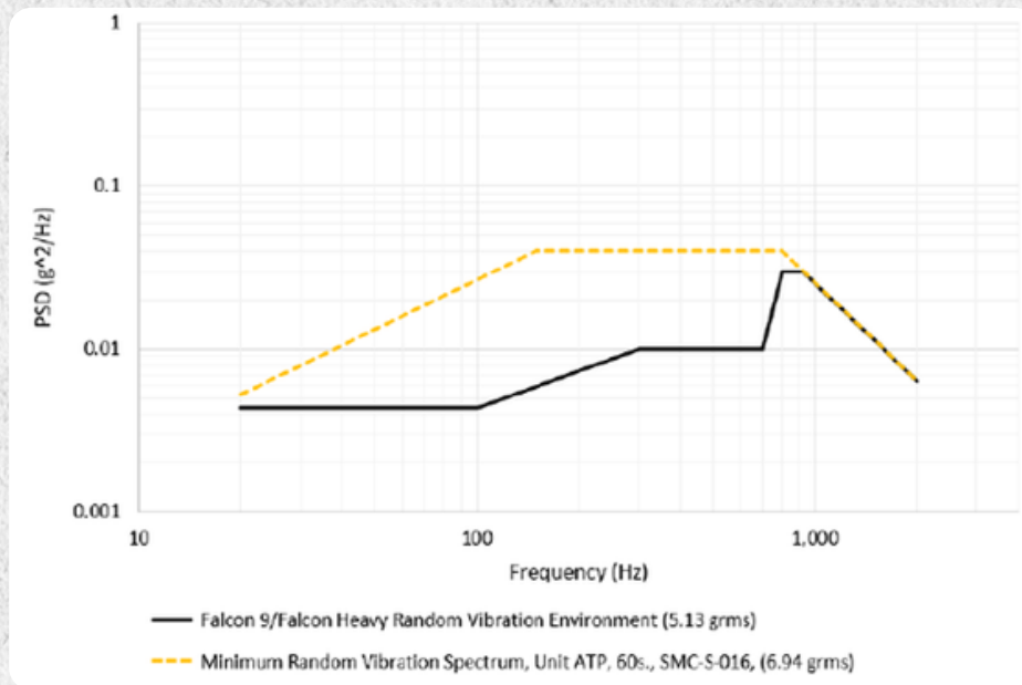
Figure 12: LLV Qualification Loads for Random Vibration
