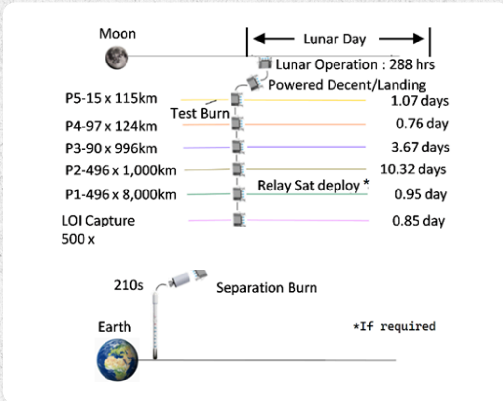
Figure 2: Example TLI Mission Trajectory
