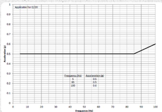
Figure 10: Lateral Equivalent Sine Environment for Falcon 9
