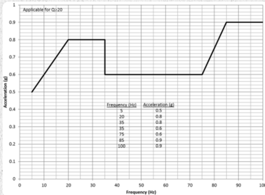
Figure 9: Axial Equivalent Sine Environment for Falcon 9
