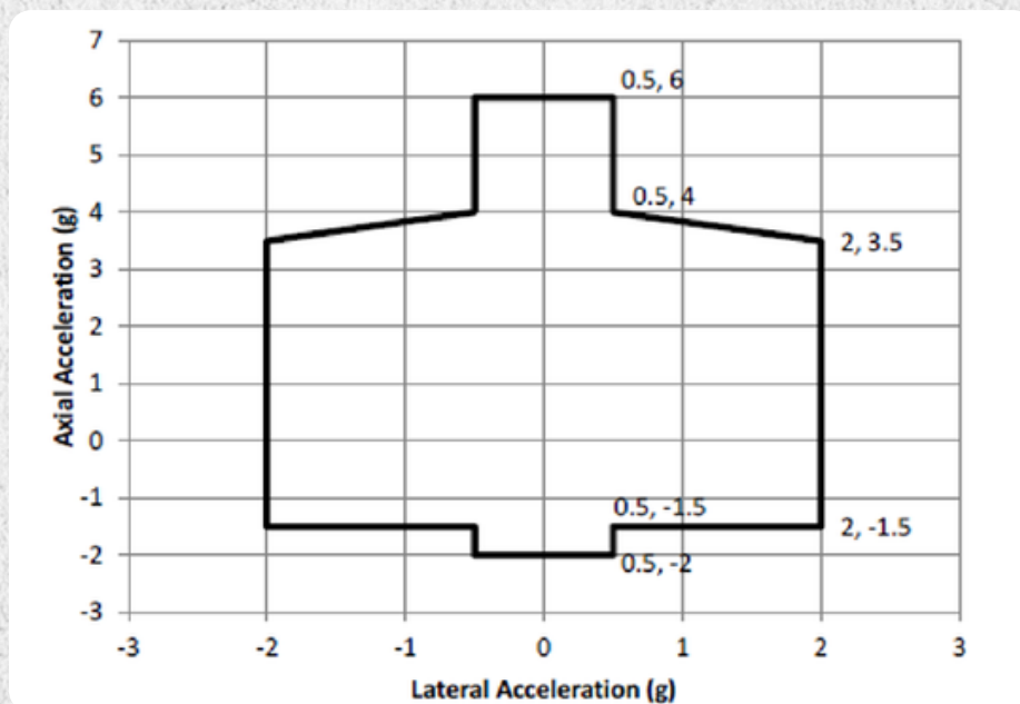
Figure 8: Design Load Factors
