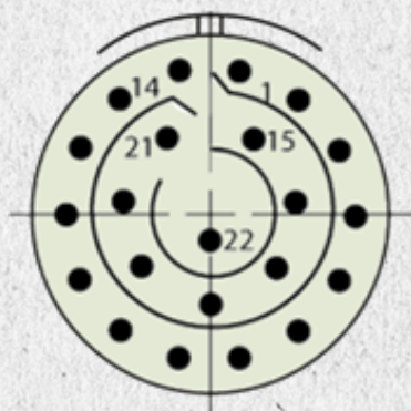
Figure 5: Data Connector Pin Definition
