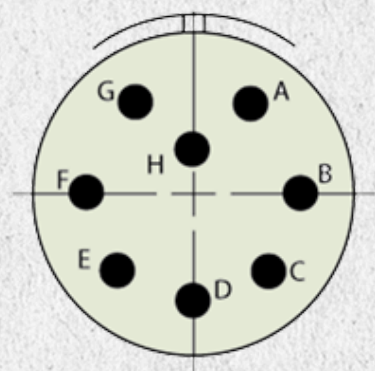
Figure 6: Power Connector Pin Definition
