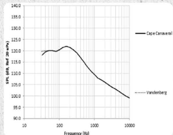
Figure 11: Payload Acoustic Maximum Predicted Environments (Full Octave)
