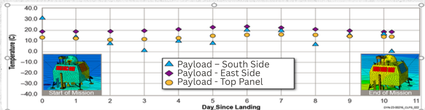
Figure 13:-Lander Temperature Profile
